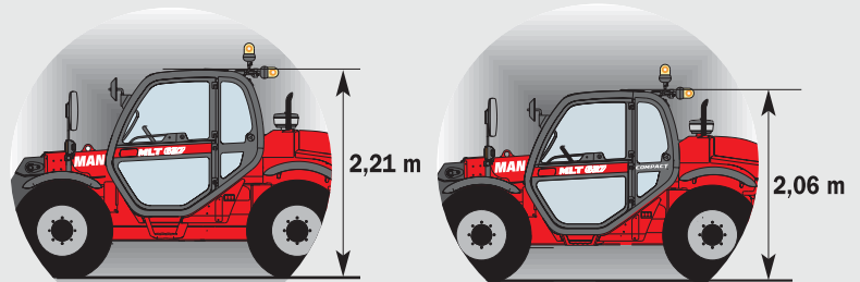
LOW PROFILE CAB "Compact" version
