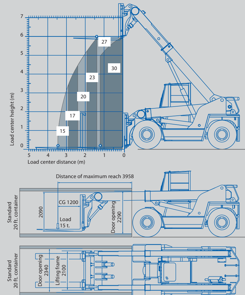
Lifting capacity diagram and working dimensions ML3012RC
